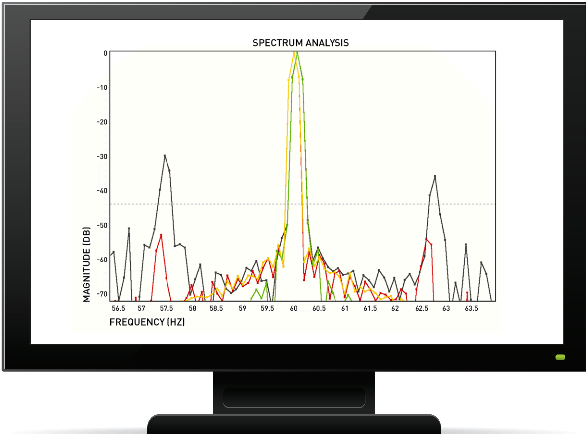
Spectrum of a running motor with three broken bars.
