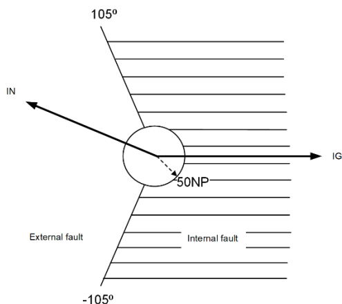
Fig. 12. Angle check in a REF element designed for low-impedance grounded systems.
