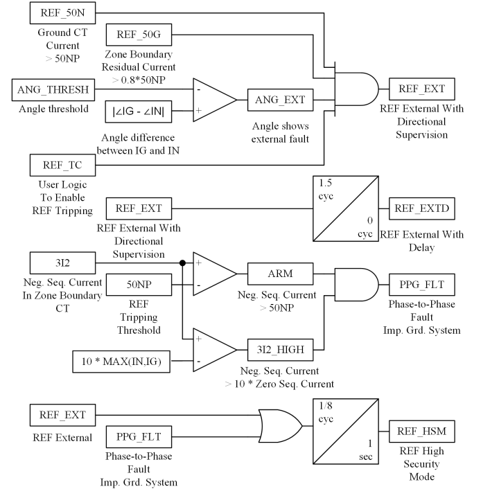
Fig. 10. REF high-security mode logic.
