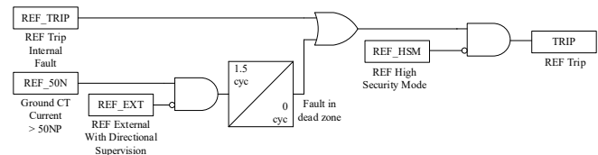
Fig. 13. Using logic to increase the dependability of the traditional REF element when the relay provides REF_EXT.
