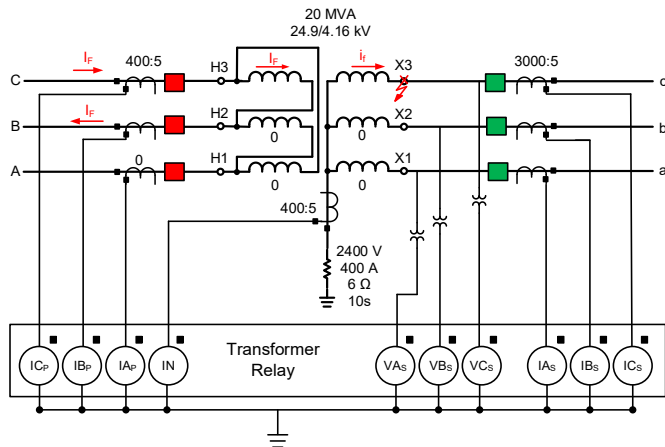
Fig. 15. Three-line diagram for case study transformer.
