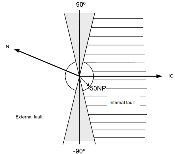
Fig. 9. Angle check with traditional REF element.
