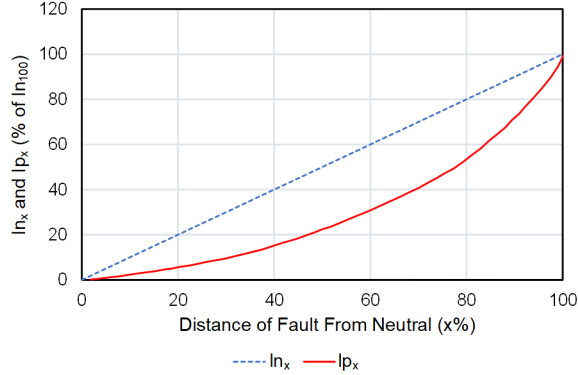
Fig. 4. I_{n_x} and I_{p_x} for ground faults along the winding of a low-impedance grounded transformer with TR = 1 [9].
